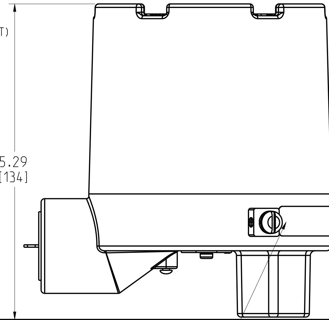
ALUMINUM CONNECTION HEAD WITH TERMINAL STRIP AND EXTENDED COVER (AT3) (COVER CHAIN OPTION AVAILABLE)
