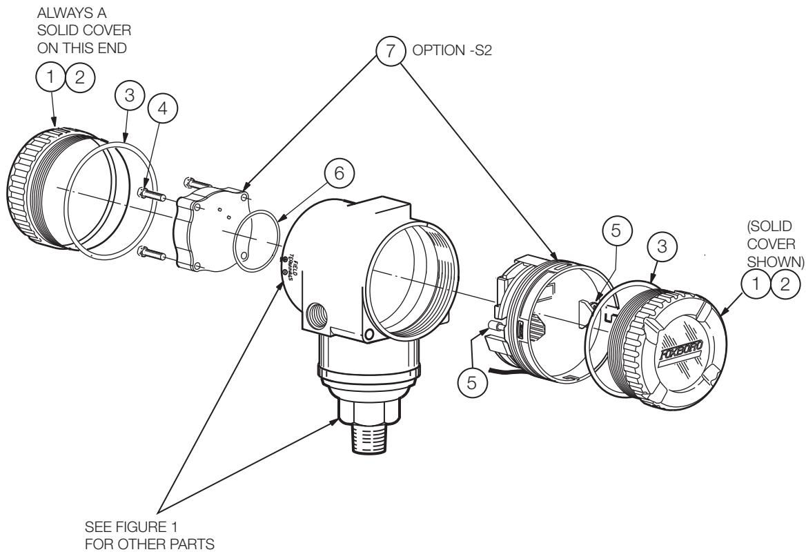
Figure 18. Optional SIL2 Transmitter for HART Versions Optional Selection -S2
