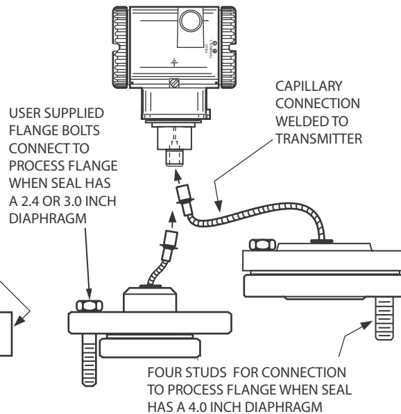
MODEL PSFAR RECESSED DIAPHRAGM-FLANGED CONNECTION REMOTE MOUNT SEALS
