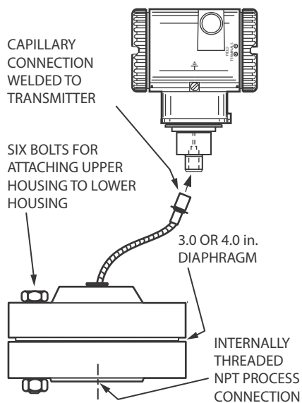
MODEL PSTAR RECESSED DIAPHRAGM THREADED CONNECTION REMOTE MOUNT SEAL
