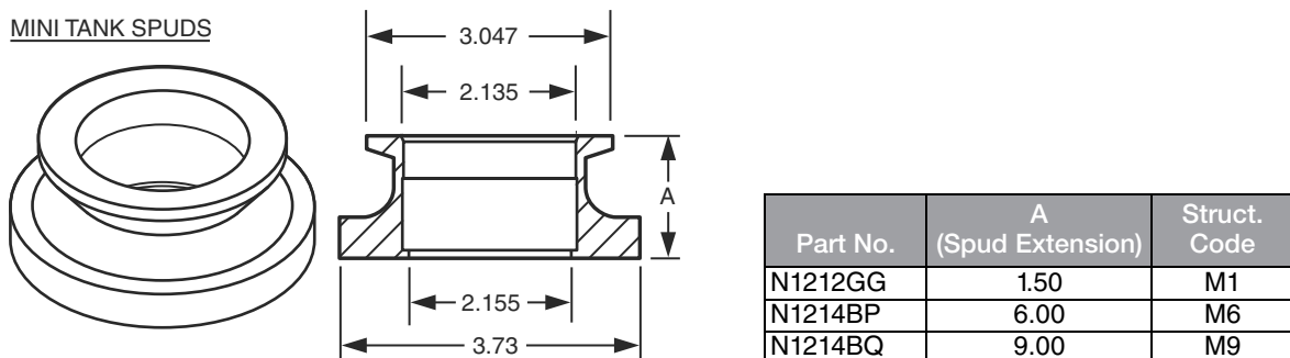
Figure 15. Accessories - Sanitary Process Connections)
