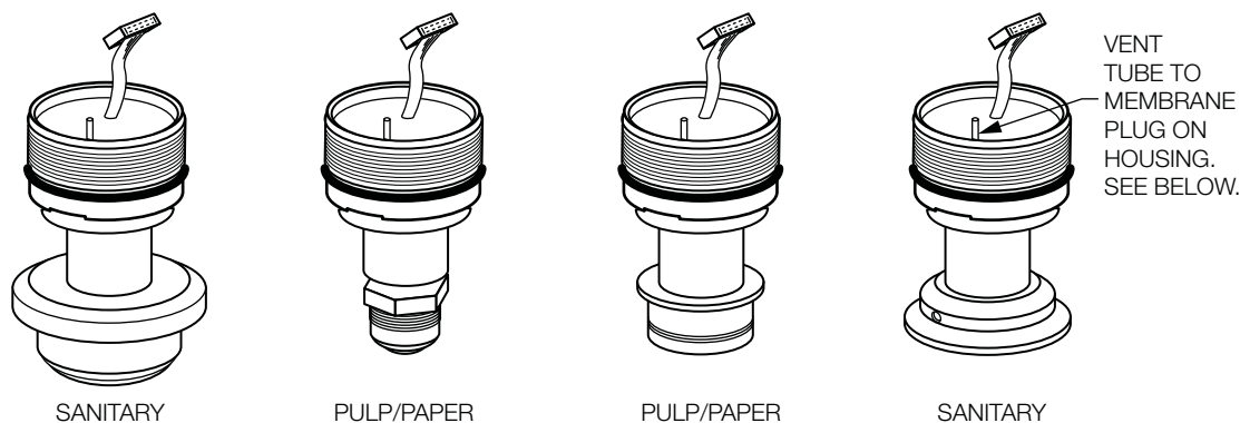
IGP10 Sanitary and Pulp/Paper Transmitters - Configurations Offered (a)
