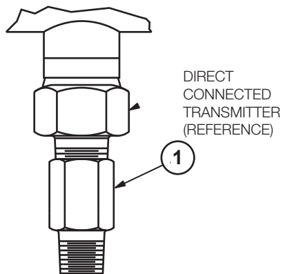
Figure 7. Optional Metric Process Connection Optional Selection -R
