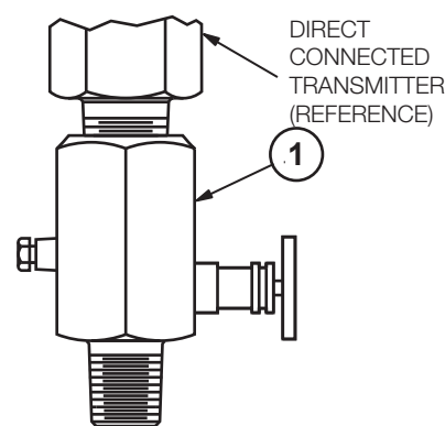
Figure 8. Optional Block and Bleed Optional Selection -V2, -V3, or -V4
