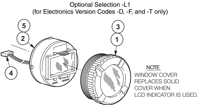
Figure 5. Optional Liquid Crystal Display (LCD) Indicator Assembly
