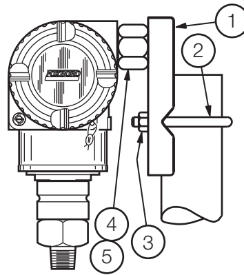
Optional Selections -M1 to -M6 (Refer to Figure 11 for part numbers of Items 1 to 5)
