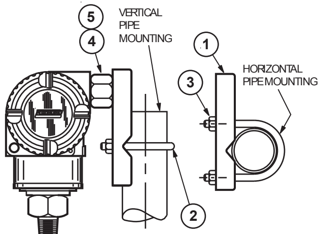
Figure 11. Optional Pipe Mounting Sets Optional Selections -M1, -M2, -M3, -M4, -M5, and -M6 (See NOTE)
