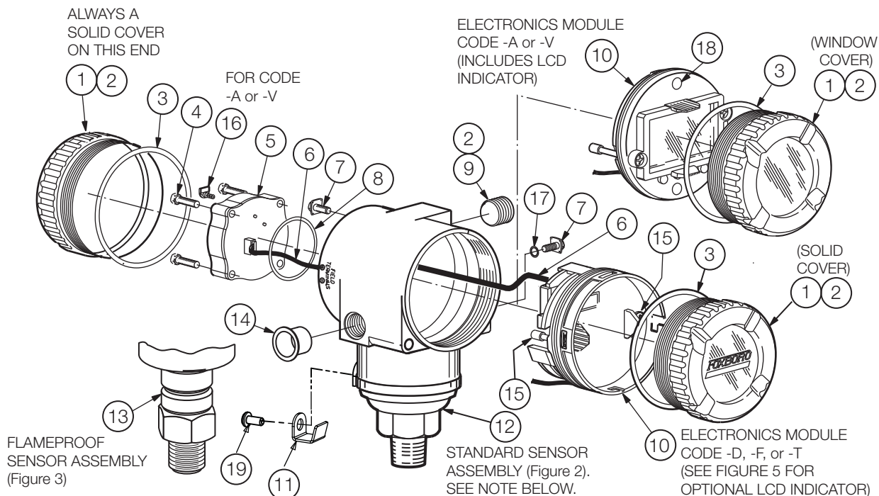
Figure 1. Transmitter Assembly
