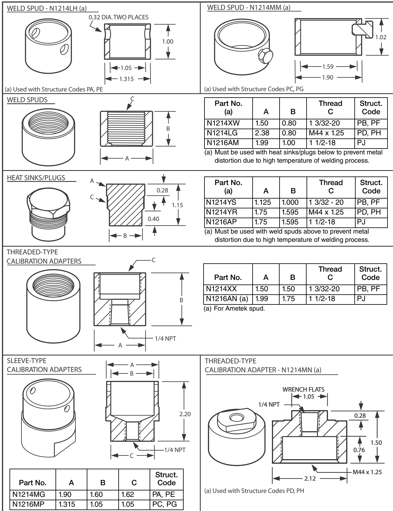
Figure 17. Accessories - Pulp and Paper Process Connections
