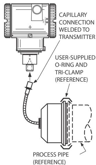
MODEL PSSCR FLUSH DIAPHRAGM SANITARY TRI-CLAMP REMOTE MOUNT SEAL
